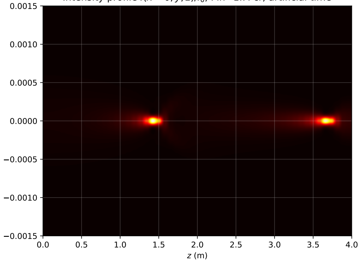
Intensity profile I(x=0, y, z)/I_0 , P_{in}=1.7P_{cr} , artificial time
